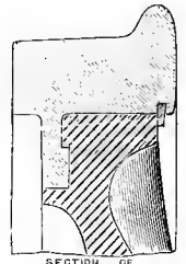
SECTION OF BOLTLESS FASTENING Fig. 5329. Section of Boltless Fastening.
